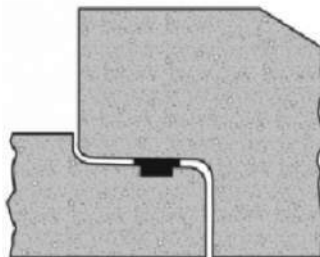
Typical cross-section opposing shoulder type bell and spigot joint with a confined o-ring rubber gasket
